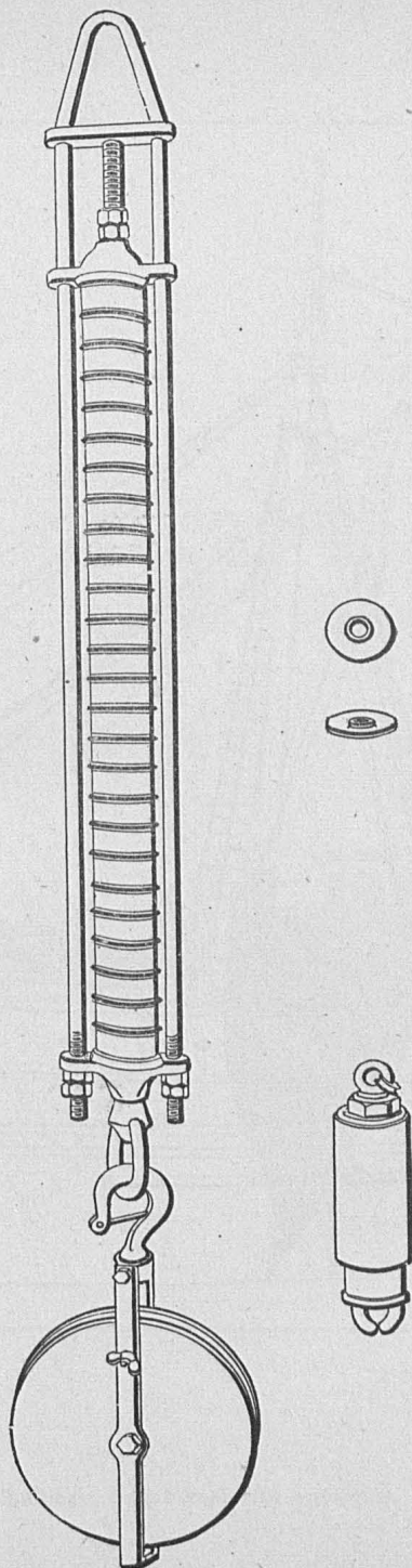
Accumulator, with dredging block hooked; safety hook; brass washer.
