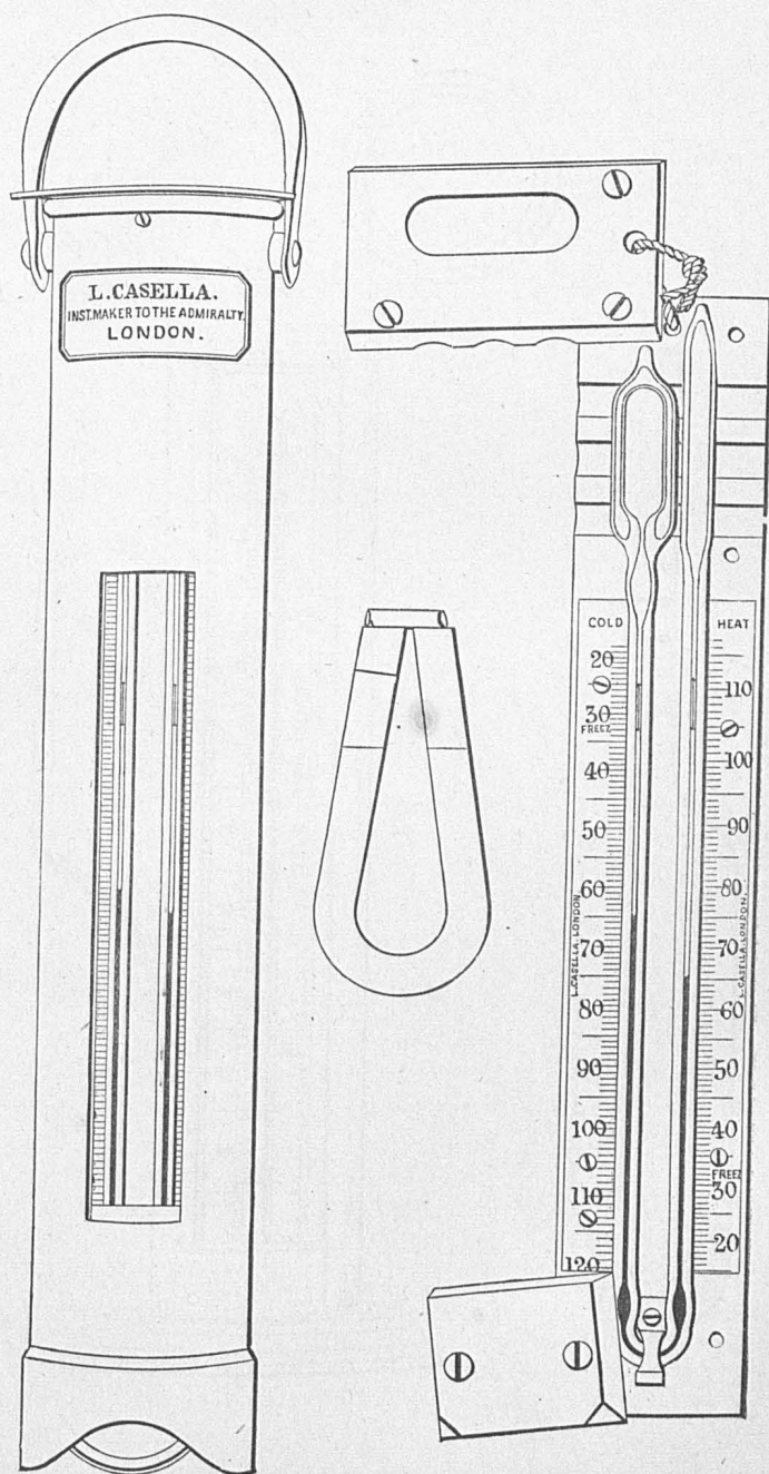
The Miller-Casella deep-sea thermometer in and out of case.
