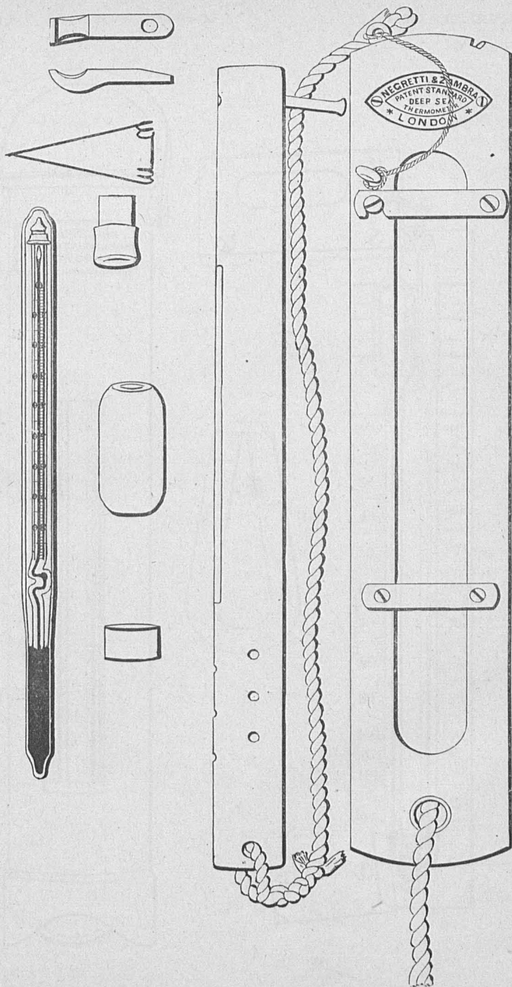
The Negretti and Zambra deep-sea thermometer, with wooden frame and metal case.
